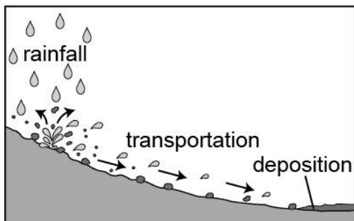
erosion process
