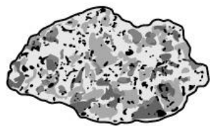
plutonic
