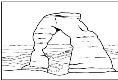
delicate arch
